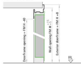
Doors without lower threshold Vertical cross section
