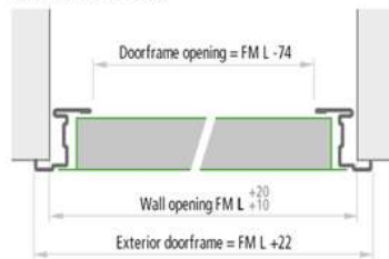
One-leaved doors Horizontal cross section
