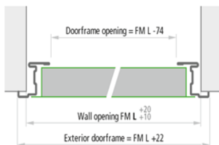
One-leaved doors Horizontal cross section
