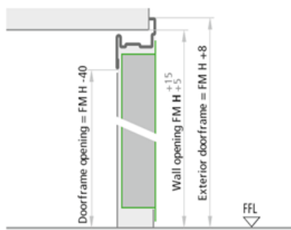
Doors without lower threshold Vertical cross section
