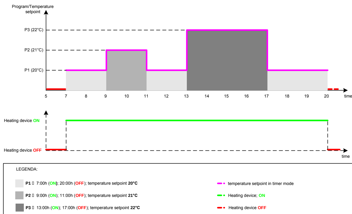
Figure 3: Programs overlapping
