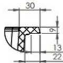
DETAIL C SCALE 2 : 5
