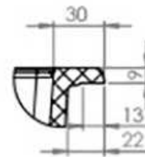
DETAIL C SCALE 2 : 5
