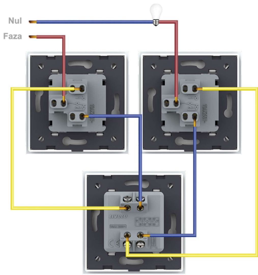
Cablare cap/scara + cap/cruce
