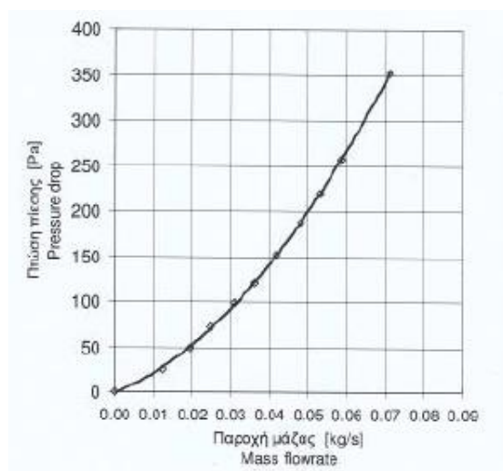
Scheme 5. Pressure loss of collectors PK SL FP 2,0 и 2,4
