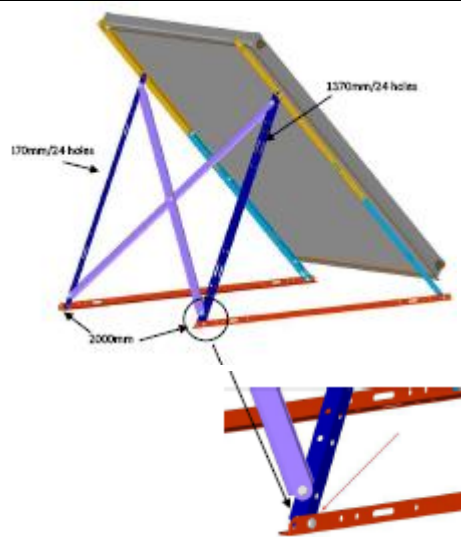
Right back side Floor L- profile 2000mm
