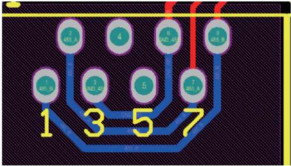
Port RS485
