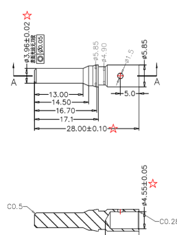
Male solid pin
