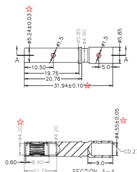
Female solid pin
