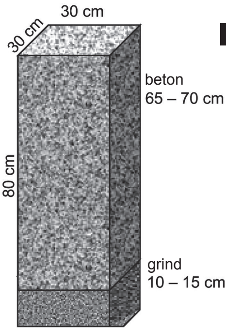
FUNDERING
