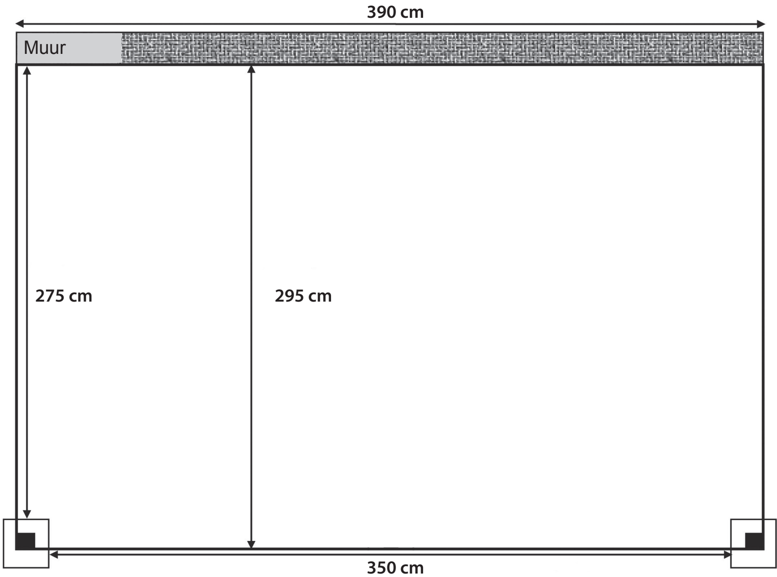
FUNDERING
