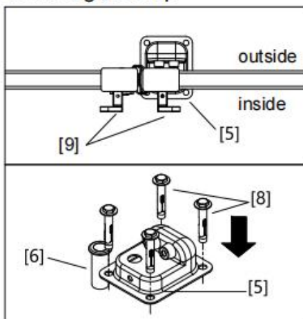
Central gate stop
