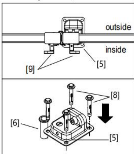
Central gate stop
