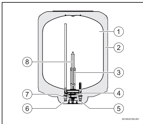
Fig. 4 Appliance components
