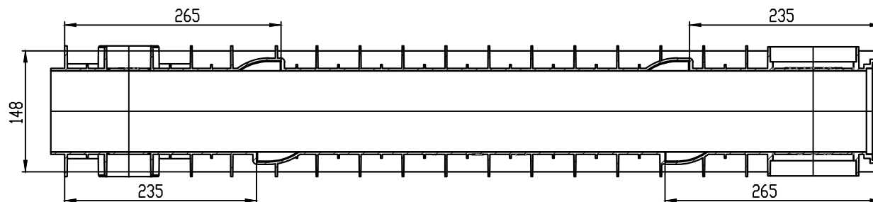
Section B-B
