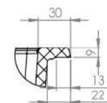
DETAIL C SCALE 2 : 5
