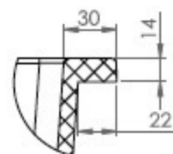
DETAIL C SCALE 2 : 5
