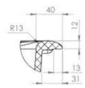
DETAIL B SCALE 2 : 5
