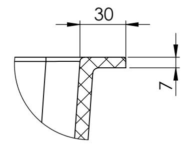
DETAIL C SCALE 2 : 5
