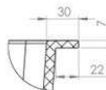
DETAIL C SCALE 2 : 5
